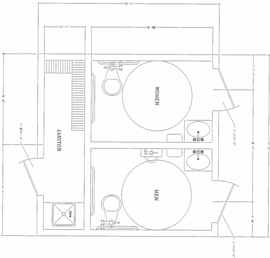
1 FLOOR PLAN S1.0 I = 1'-0"
